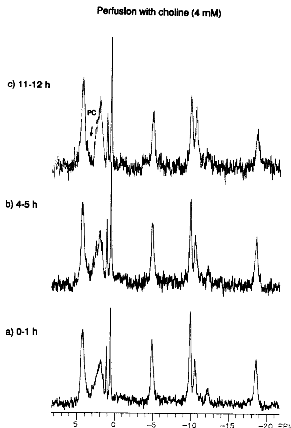
Fig.3. ^{31}\text{P} NMR spectra of TILs perfused with IMEM containing 4 mM choline (for acquisition parameters see section 2; LB = 5 Hz).
